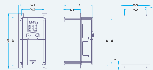
18.5-30kW Flange mounting Installation diagram
