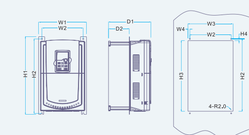
11-15kW Flange mounting installation diagram
