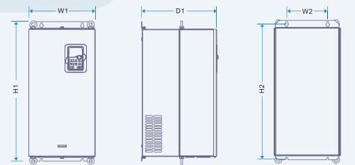
18.5-55kW Installation
