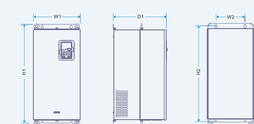
132-200kW Flange mounting Installation diagram
