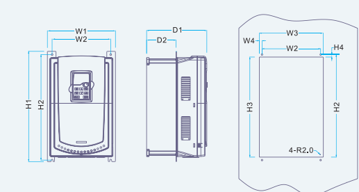
37-110kW Flange mounting Installation diagram
