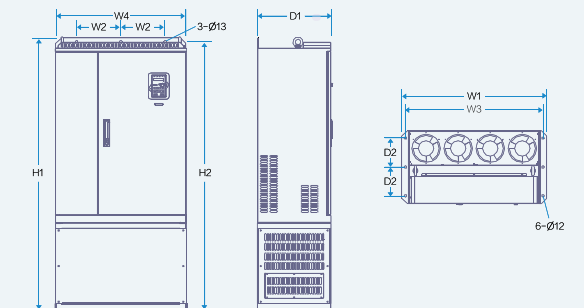
355-500kW Floor mounting Installation diagram
