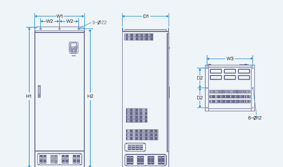
355-500kW Floor mounting Installation diagram
